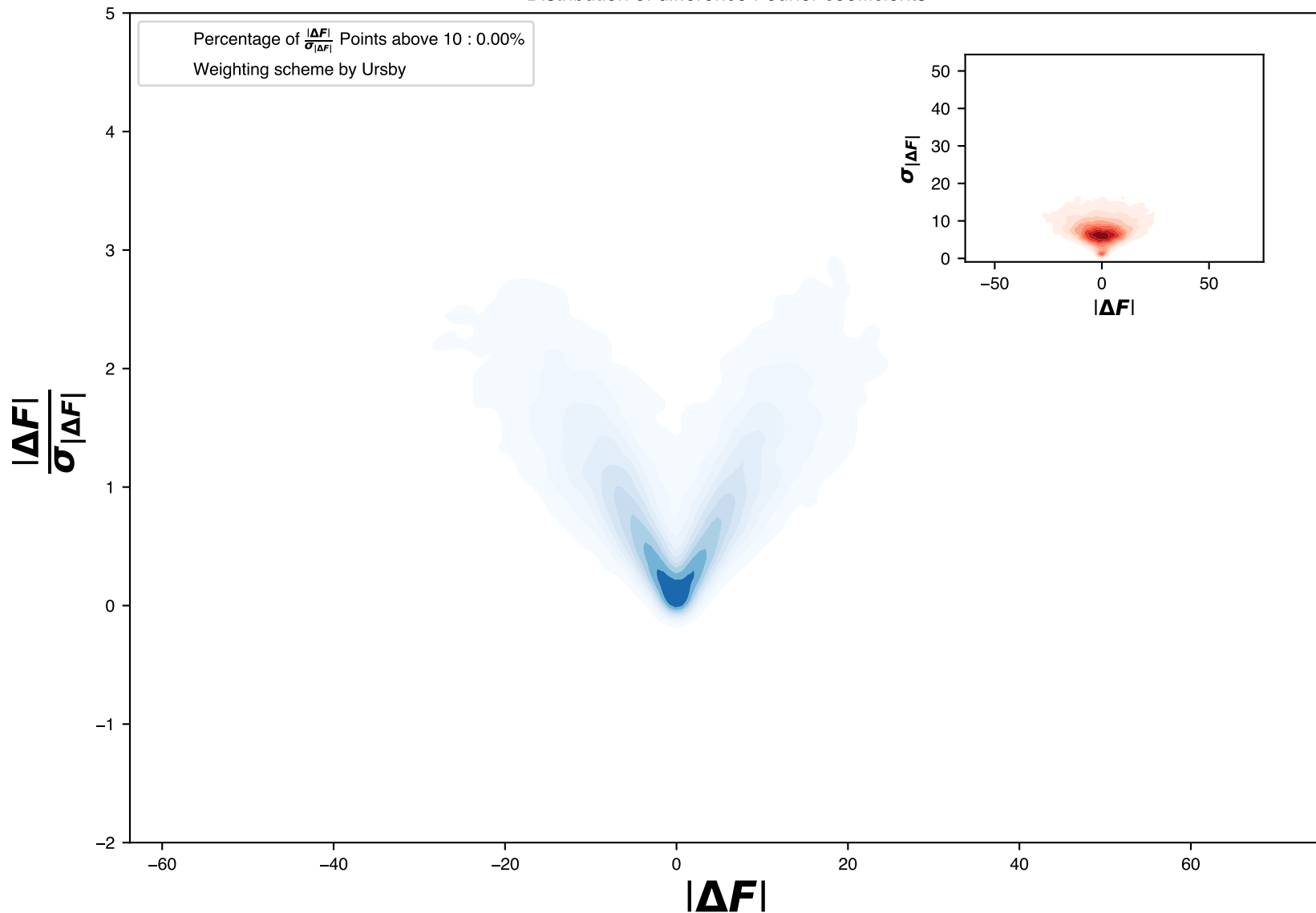
Distribution of difference Fourier coefficients
