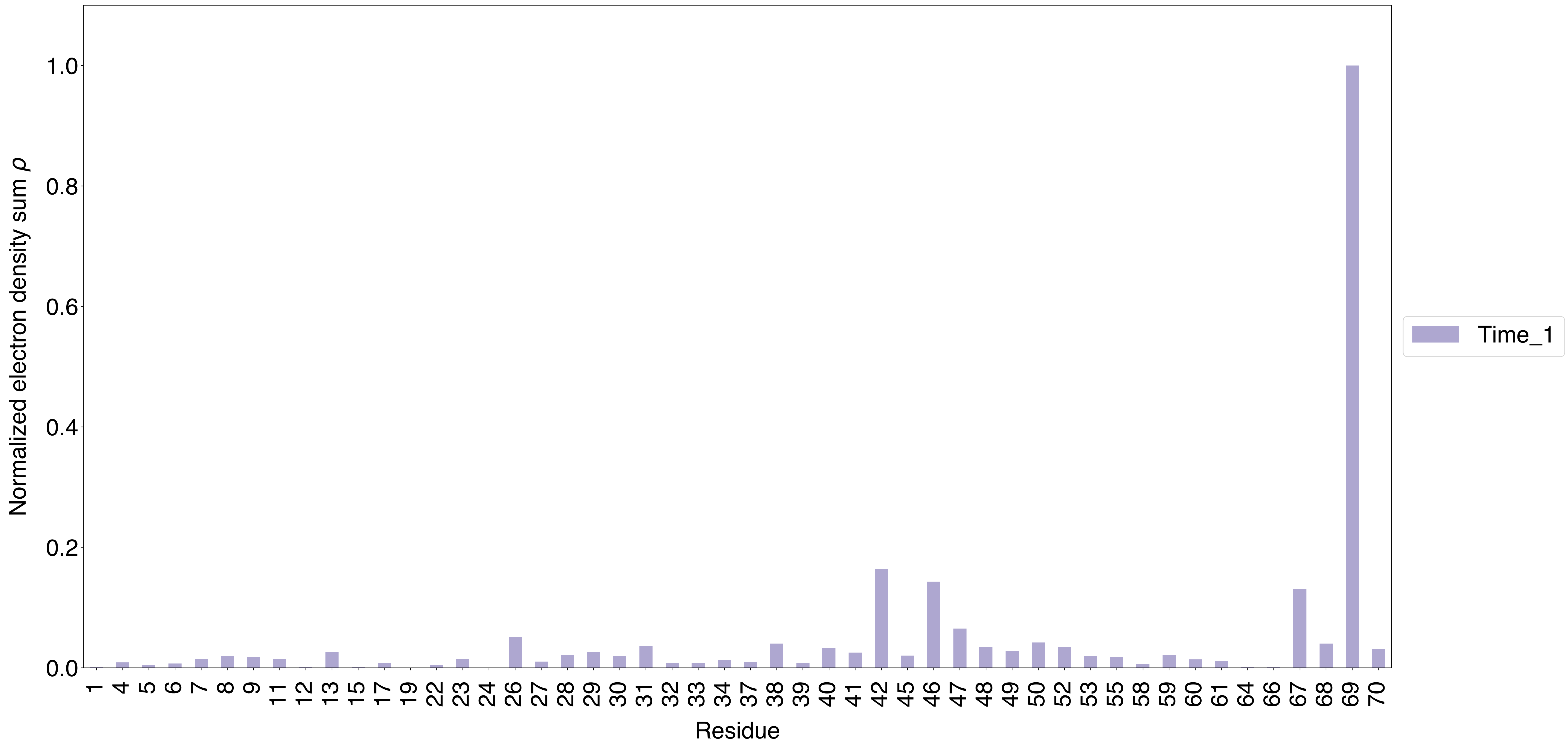
Variation of normalized electron sum \rho over time
